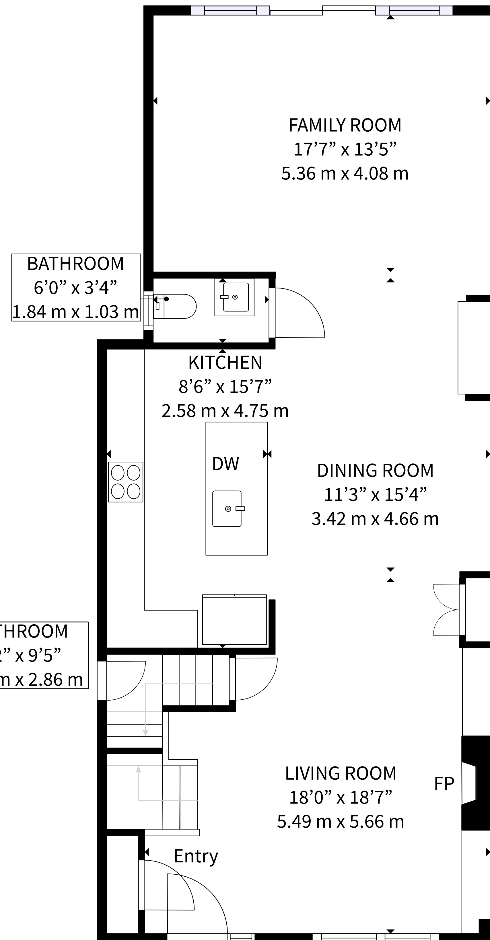
FLOOR 1
