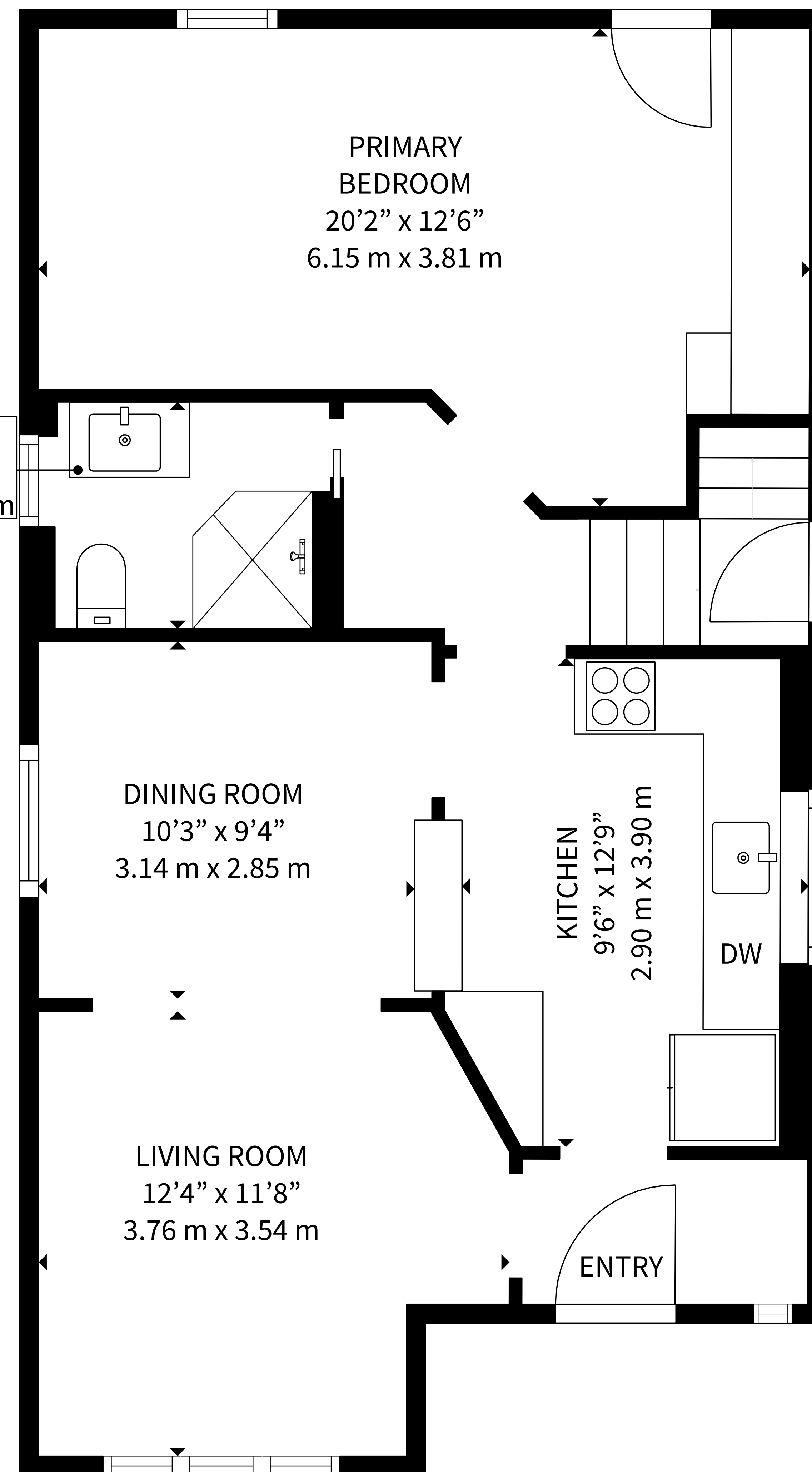
FLOOR 1
