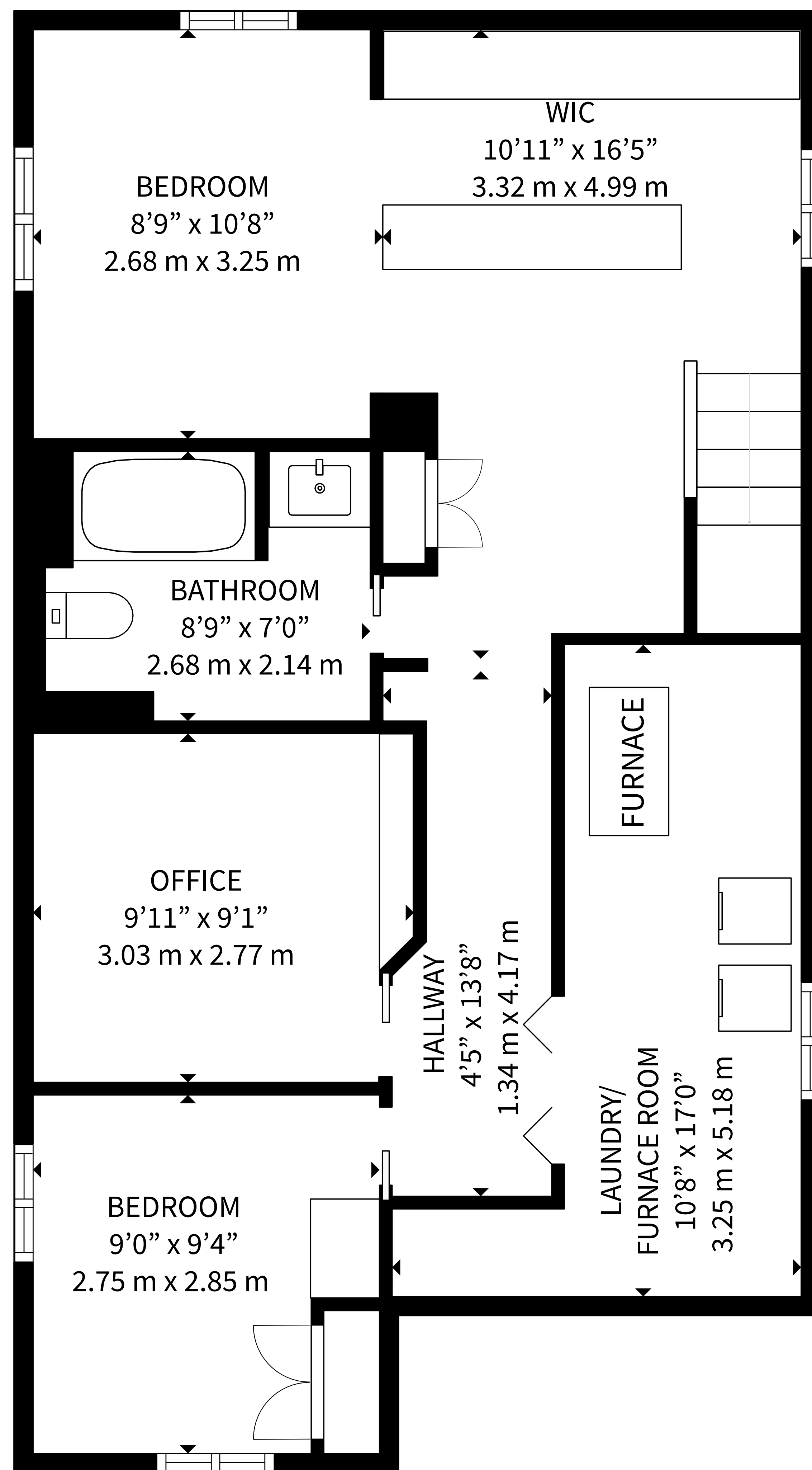
BASEMENT
